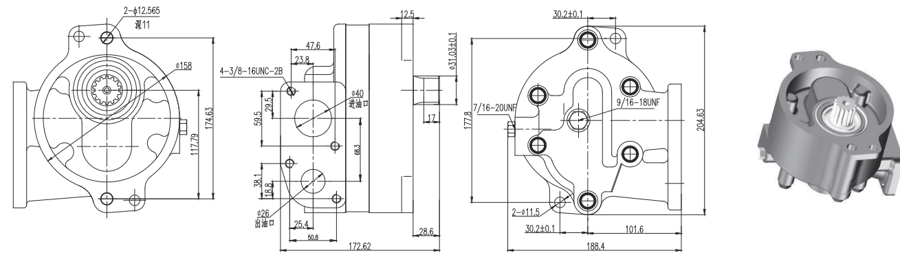
3S4386 Dimensions
