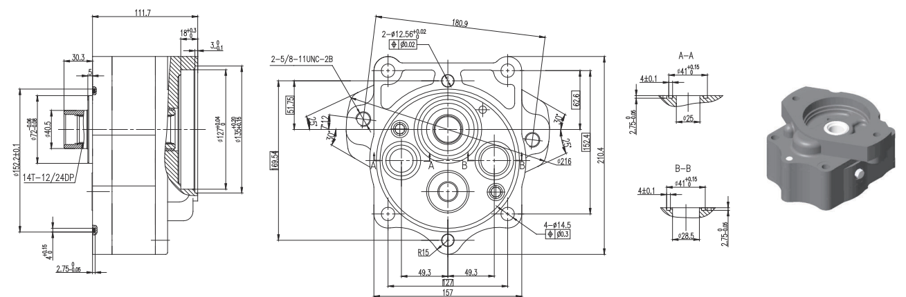
7S4629 Dimensions
