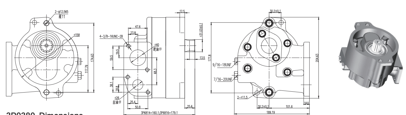
3P0380 Dimensions
